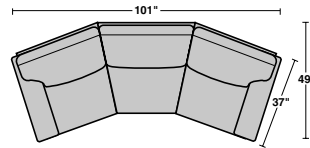
Overall dimensions of 3979-323 conversation sofa
